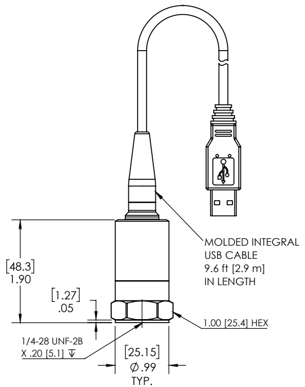
Model 333D01
